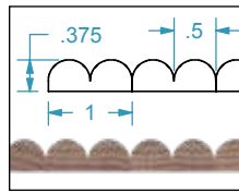
STYLE 105 1/2" BEAD FLEXIBLE TAMBOUR - .375" THICK
