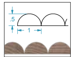
STYLE 104 1" BEAD FLEXIBLE TAMBOUR - .5" THICK
