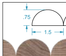
STYLE 106 1.5" BEAD FLEXIBLE TAMBOUR - .75" THICK
