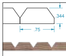
STYLE 202 3/4" BEVEL FLEXIBLE TAMBOUR -.344" THICK
