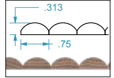
STYLE 101 3/4" BEAD FLEXIBLE TAMBOUR - .313" THICK
