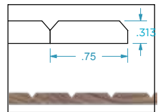
STYLE 201 3/4" BEVEL FLEXIBLE TAMBOUR - .313" THICK
