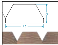
STYLE 207 1-1/2" BEVEL FLEXIBLE TAMBOUR- .75" THICK
