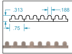
STYLE 103 3/16" BEAD FLEXIBLE TAMBOUR - .313" THICK
