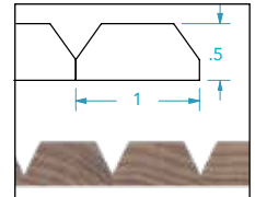
STYLE 204 1" BEVEL FLEXIBLE TAMBOUR - .5" THICK
