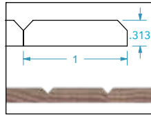
STYLE 203 1" BEVEL FLEXIBLE TAMBOUR - .313" THICK
