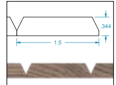
STYLE 206 1-1/2" BEVEL FLEXIBLE TAMBOUR- .344" THICK
